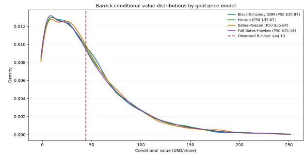
Gold-price layer only: conditional transfer of GLOD distributional shape to gold USD/oz. Common deterministic: Team 4 production/cost vectors and Team 5 DCF/WACC; densities use the pooled P0.5–P99.5 display range.
