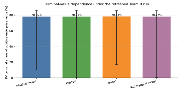
Figure 9 (continued). Present-value terminal share on positive-EV paths. Refreshed medians are 78.26% for Black–Scholes, 78.31% for Heston, 78.43% for Bates and 78.27% for Full Bates–Hawkes; bars show the P10–P90 range.
